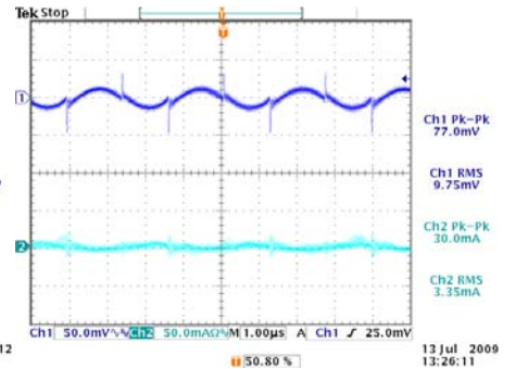
Input/Output ripples of CBQ10048S5V0-LabcXXX ( V_{IN} : 48V, Load: 25A, L_{IN} =10uH, C_{IN} =100uH)
