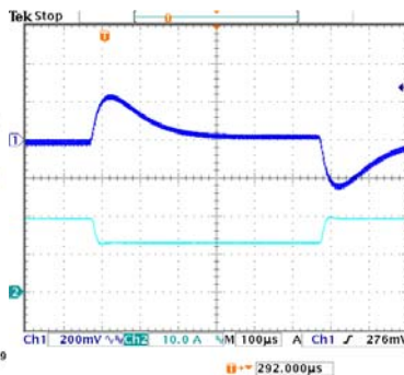
Transient response of CBQ10024S3V3-LabcXXX ( V_{IN} : 24V, Load: 20A/12.5A@2.5A/ \mu S)
