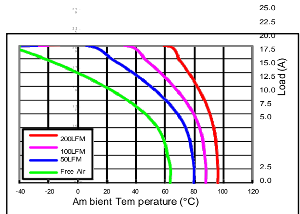
Derating curves of CBQ10048S5V0-LabcXXX for T_c = 110^\circ\text{C}
