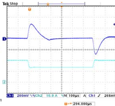
Transient response of CBQ10048S5V0-LabcXXX ( V_{IN} : 48V, Load: 20.5A/13.0A@2.5A/ \mu S)
