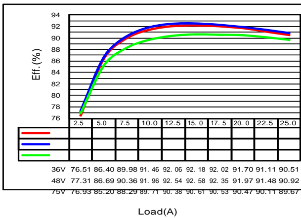
Efficiency plot of CBQ10048S5V0-LabcXXX
