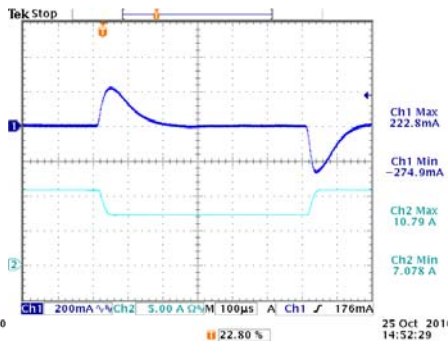
Transient response of COQ48120abcd-14XXX ( V_{IN} : 48V, Load: 10.5A/7.5A@2.5A/µs)
