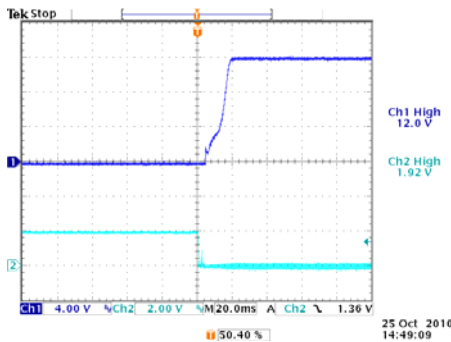
Start-up waveform of COQ48120abcd-14XXX ( V_{IN} : 48V, Load: 14A)
