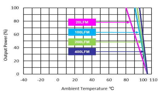
MJW15-24S24, MJW15-48S24 Derating Curve with Heatsink
