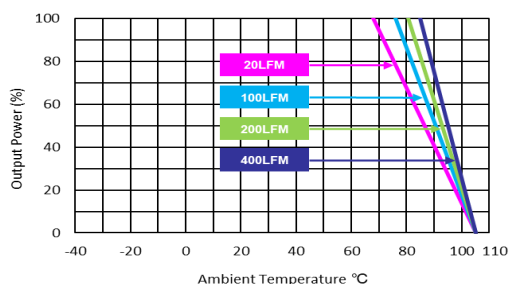
MJW15-24S05, MJW15-48S05 Derating Curve without Heatsink
