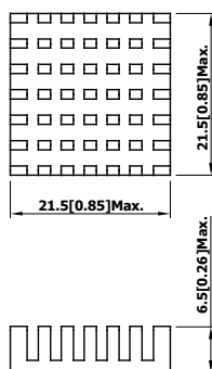
Order Code For Heatsink kit (including: Heatsink x1, Clamp x 2, Thermal Pad x1)
