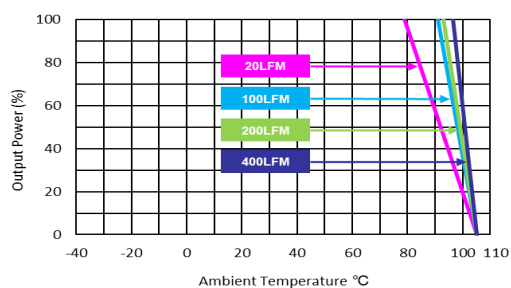
MJW15-48S033 Derating Curve with Heatsink
