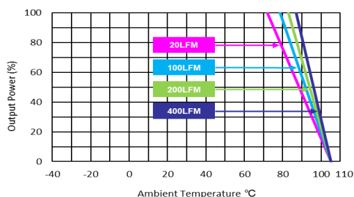
MJW15-12S033, MJW15-24S033 Derating Curve without Heatsink
